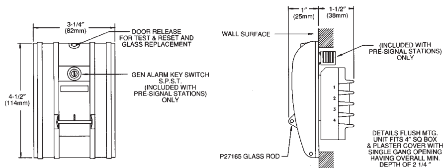
FLUSH INSTALLATION USING P-024900 STEEL BOX
