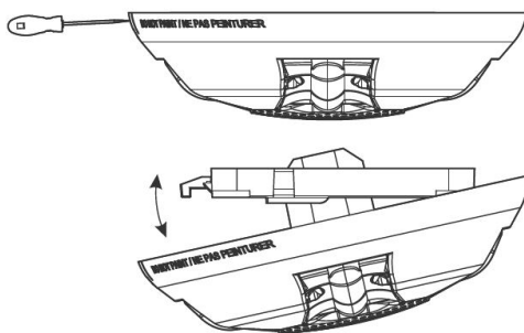
Removing Device
