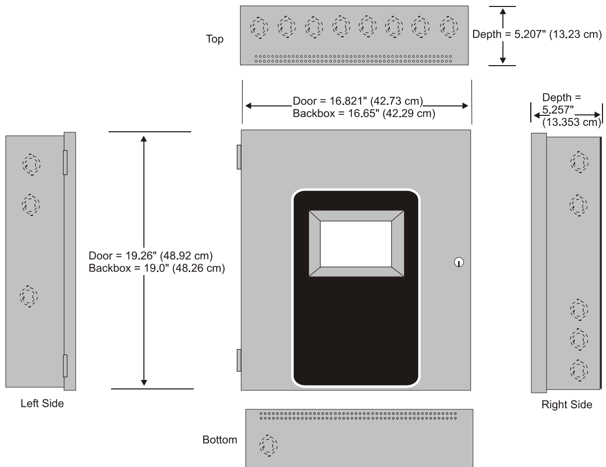
Cabinet Measurements
